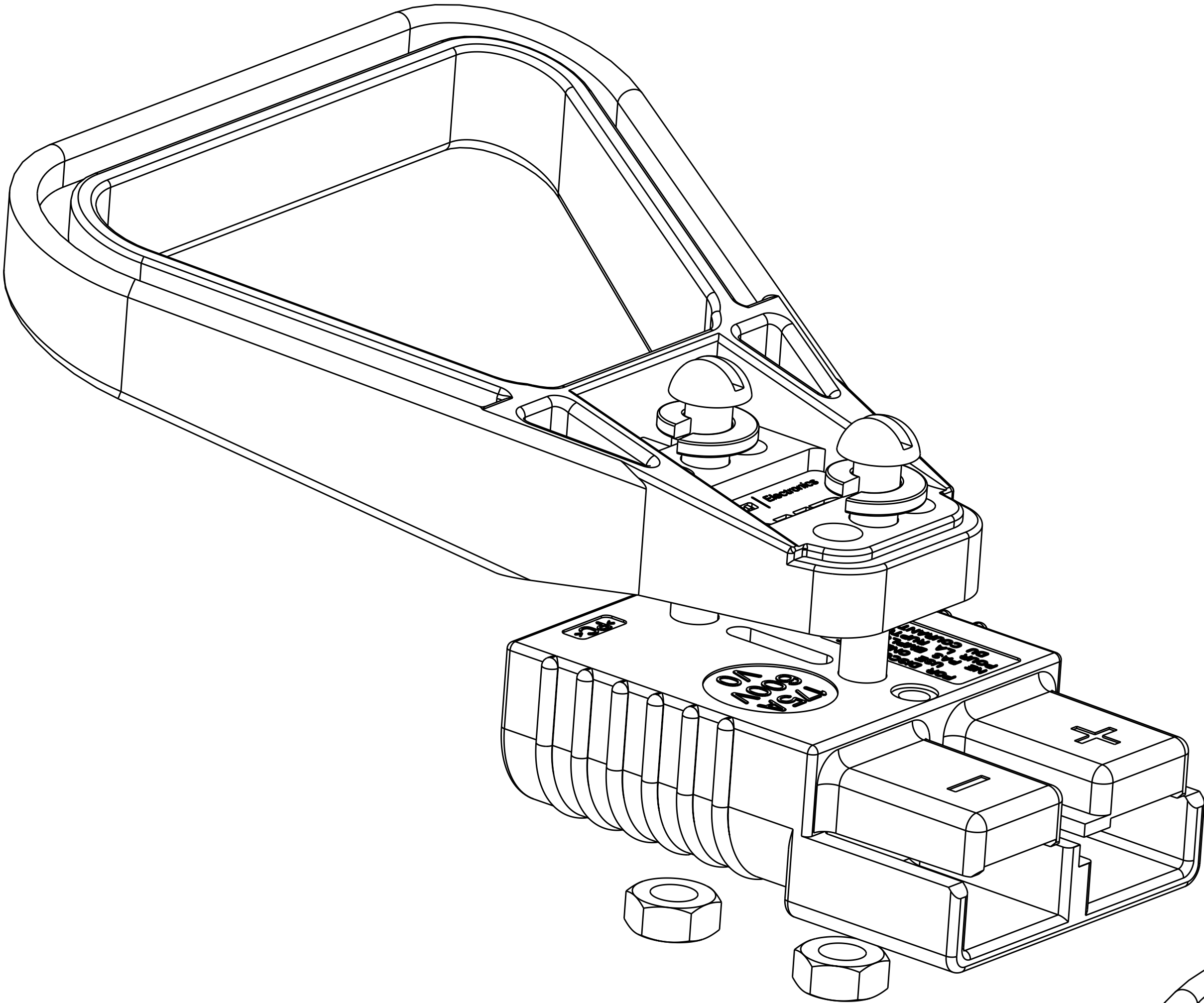
175A HOUSING SHOWN SCALE 2:1
