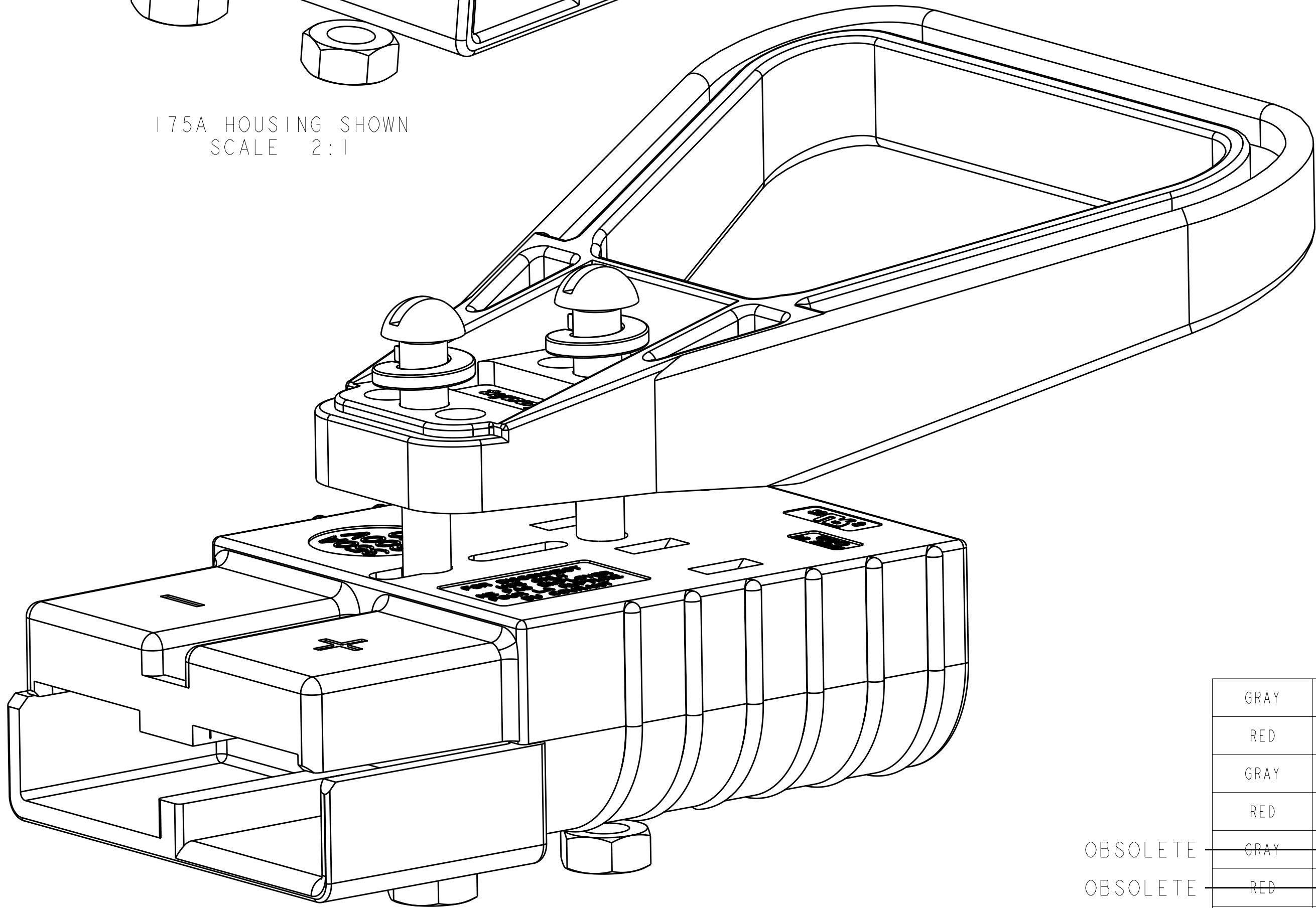
350A HOUSING SHOWN SCALE 2:1
