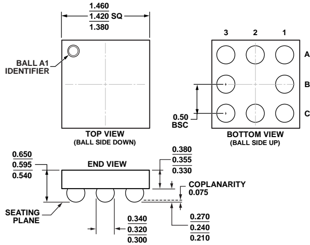
Figure 61. 8-Ball Wafer Level Chip Scale Package [WLCSF] (CB-8-2) Dimensions shown in millimeters
