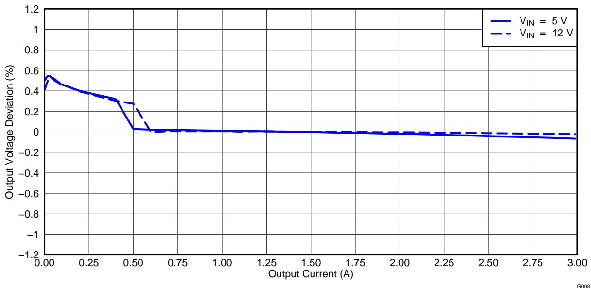
Figure 6. TPS54395EVM Converter 2 Load Regulation
