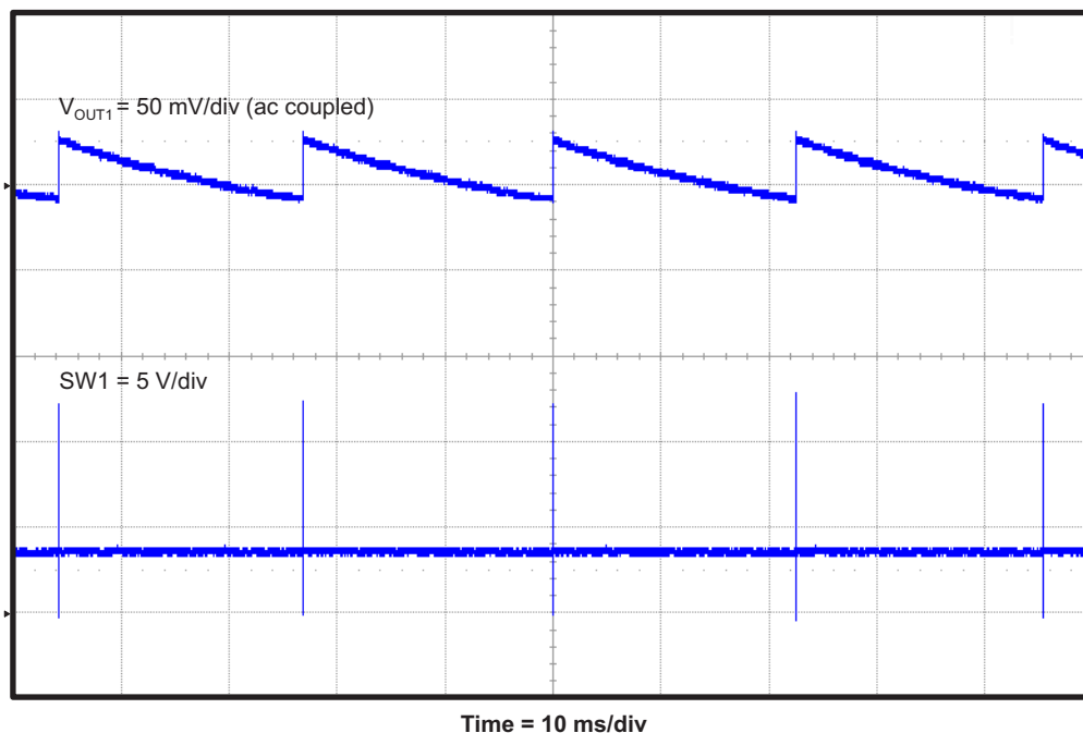
Figure 12. TPS54395EVM Converter 1 Eco-mode™ Output Voltage Ripple at No Load
