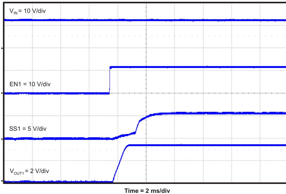
Figure 17. TPS54395EVM Start-Up Relative to EN1
