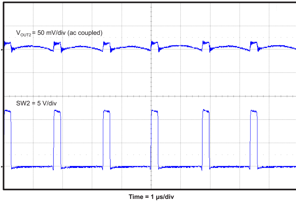
Figure 13. TPS54395EVM Converter 2 Output Voltage Ripple
