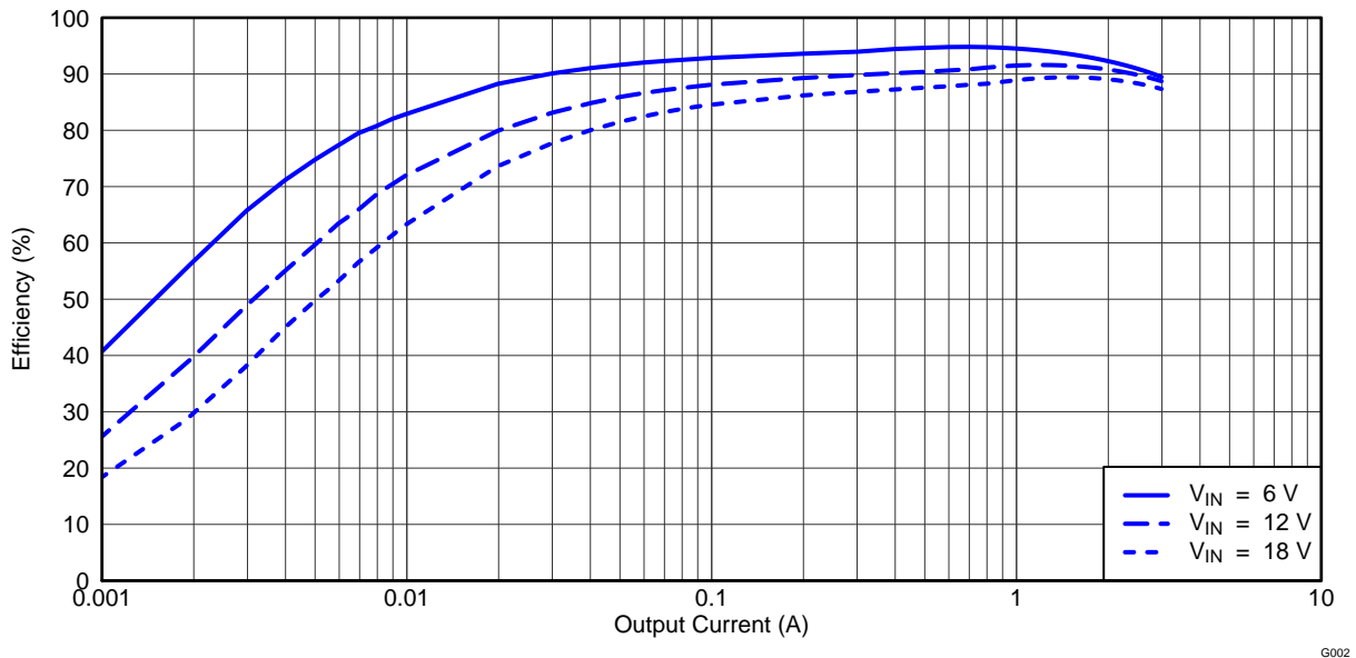
Figure 2. TPS54395EVM Converter 1 Light Load Efficiency
