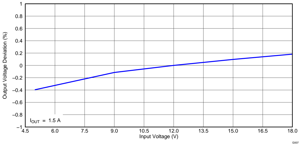
Figure 8. TPS54395EVM Converter 2 Line Regulation
