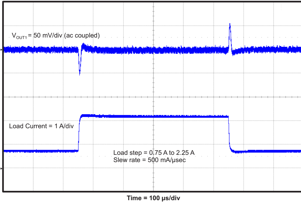
Figure 9. TPS54395EVM Converter 1 Load Transient Response
