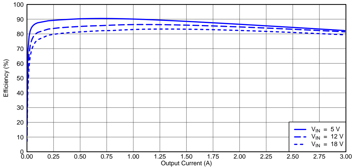
Figure 3. TPS54395EVM Converter 2 Efficiency
