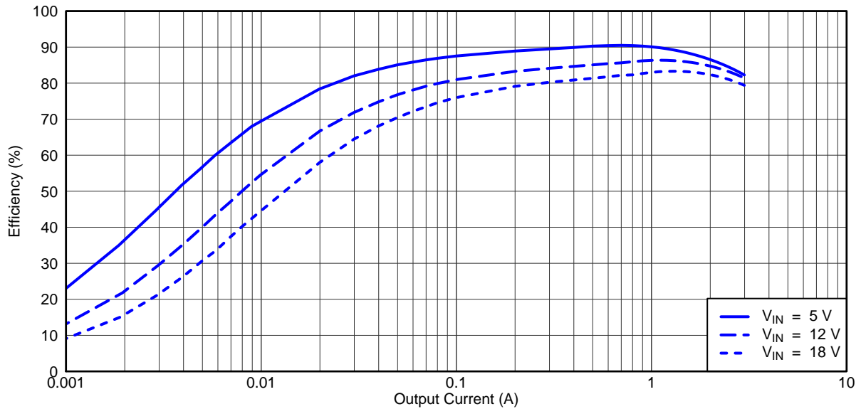
Figure 4. TPS54395EVM Converter 2 Light Load Efficiency
