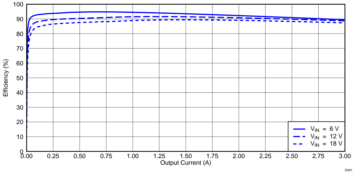
Figure 1. TPS54395EVM Converter 1 Efficiency
