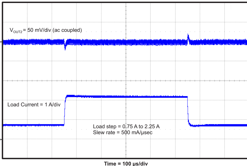
Figure 10. TPS54395EVM Converter 2 Load Transient Response
