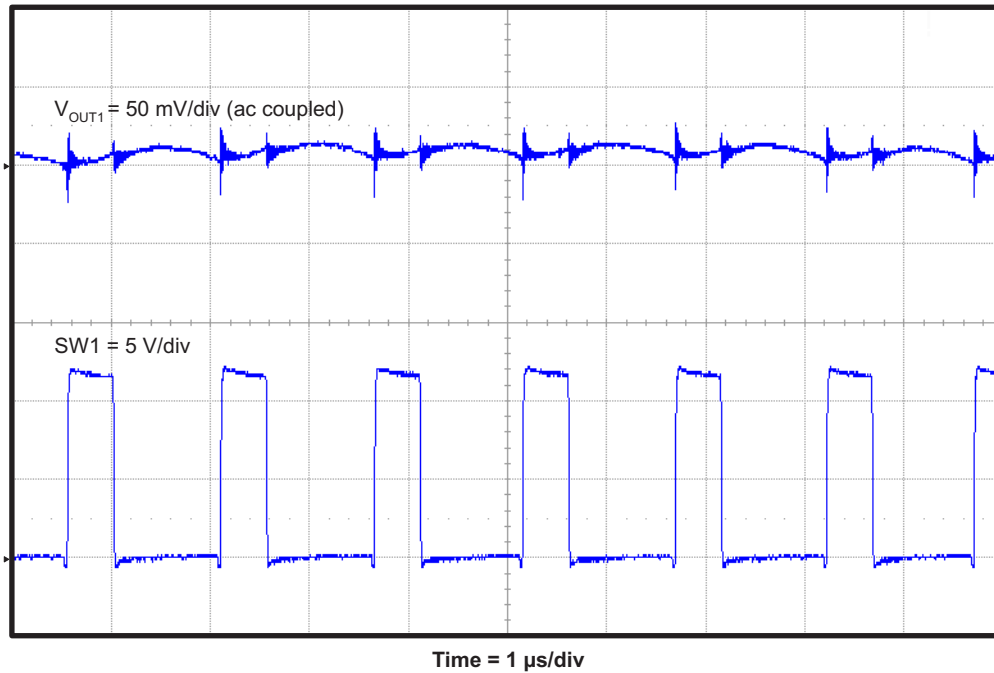
Figure 11. TPS54395EVM Converter 1 Output Voltage Ripple
