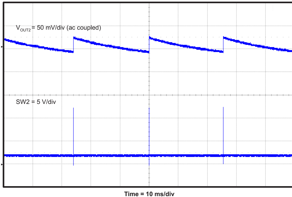
Figure 14. TPS54395EVM Converter 2 Eco-mode™ Output Voltage Ripple at No Load
