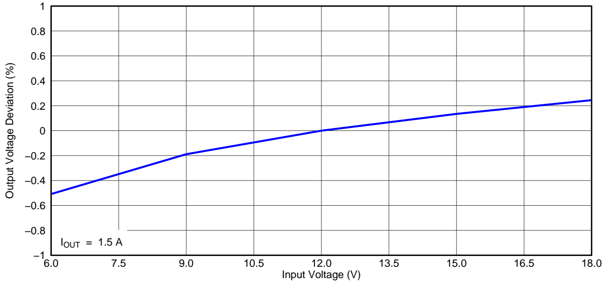
Figure 7. TPS54395EVM Converter 1 Line Regulation
