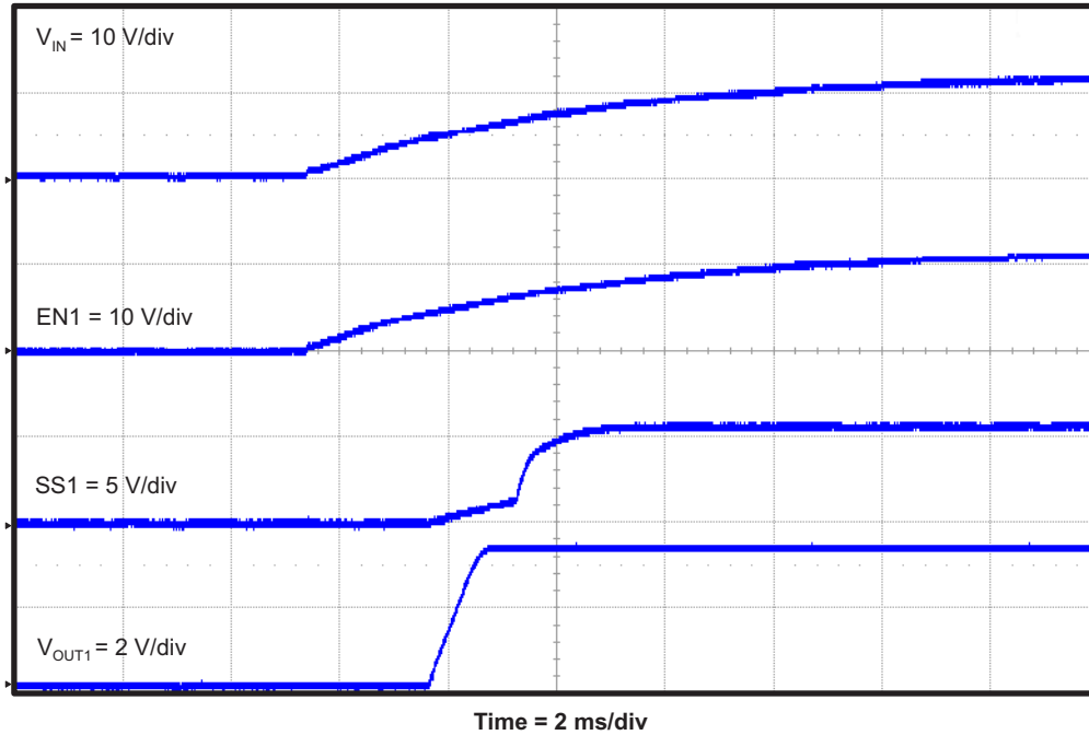
Figure 16. TPS54395EVM Converter 1 Start-Up Relative to V_{IN}
