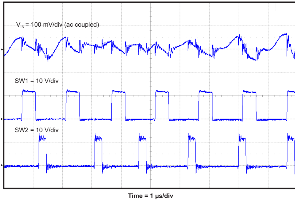
Figure 15. TPS54395EVM Input Voltage Ripple
