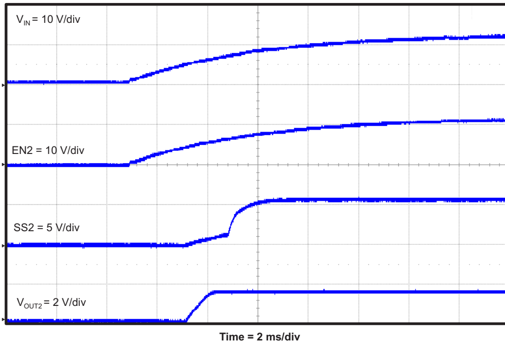
Figure 18. TPS54395EVM Converter 2 Start-Up Relative to V_{IN}
