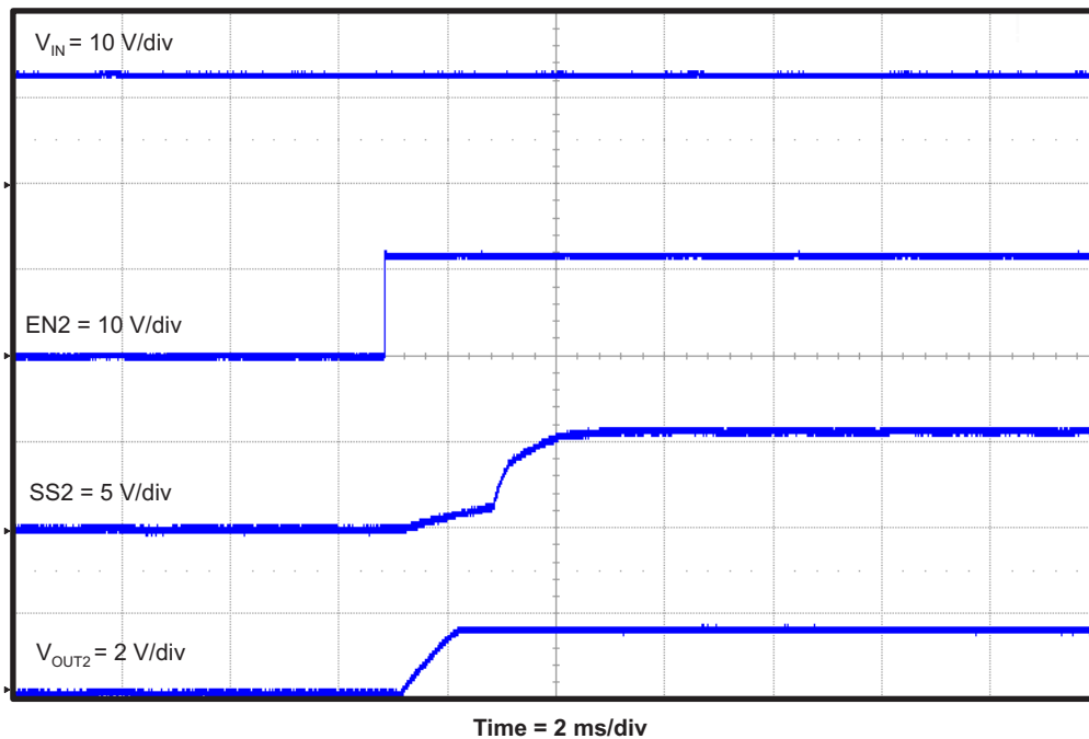
Figure 19. TPS54395EVM Start-Up Relative to EN2
