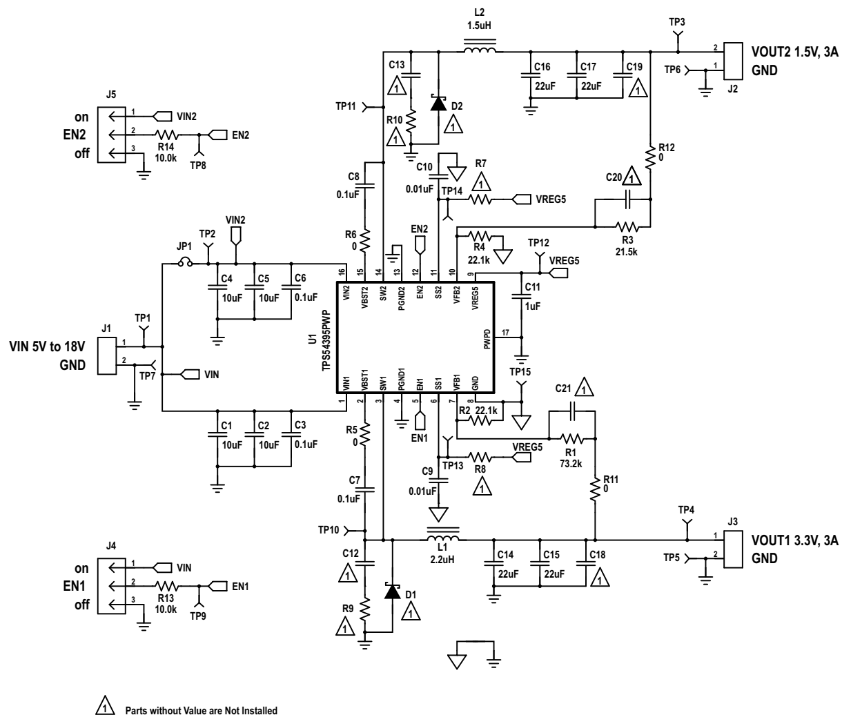
Figure 26. TPS54395EVM Schematic Diagram
