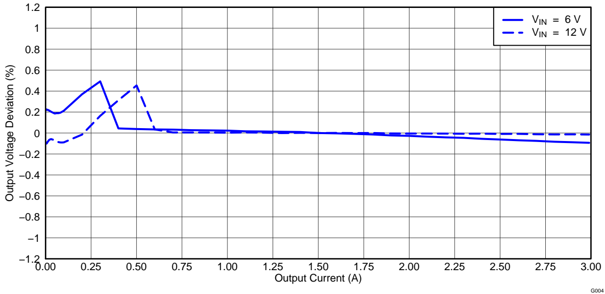
Figure 5. TPS54395EVM Converter 1 Load Regulation
