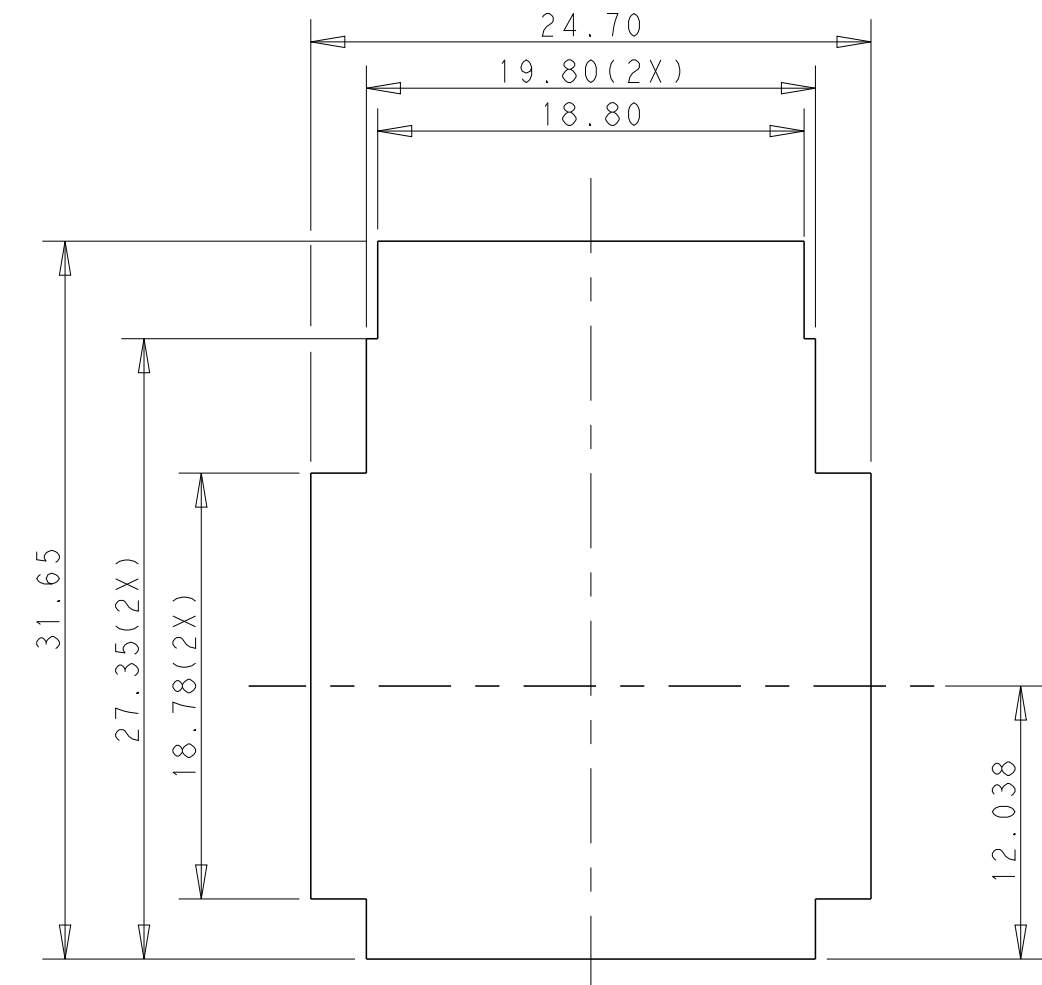
RECOMMENDED PANEL OPENING DIMENSIONS FOR CAP HOUSING 3*3 POSITION (TOLERANCE: ±0.15mm )
