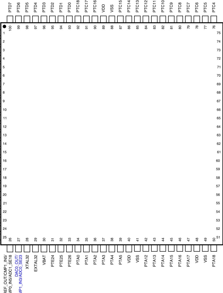
Figure 28. K20 100 LQFP Pinout Diagram
