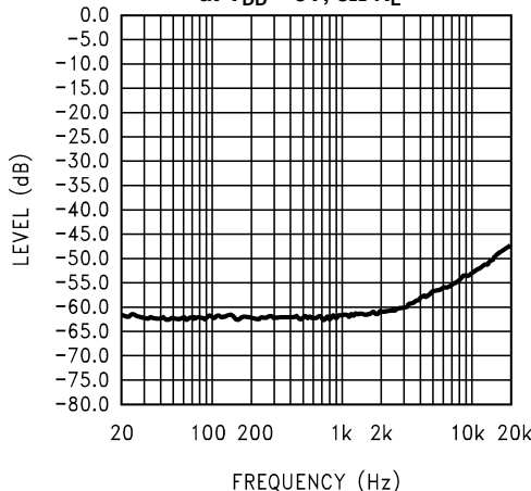
Figure 15. Input Floating
