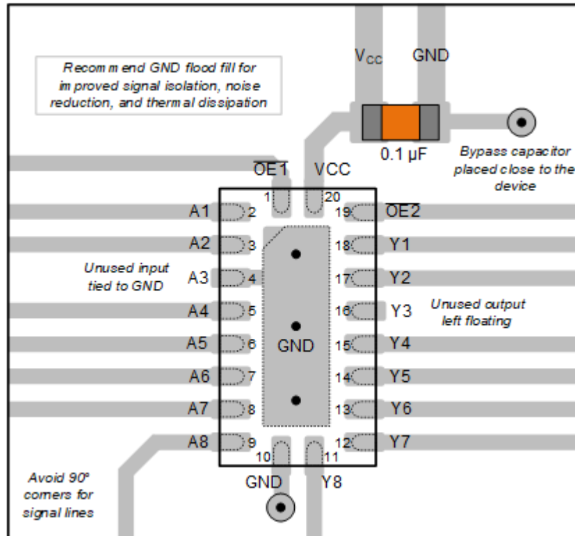
Figure 9-1. Layout Diagram
