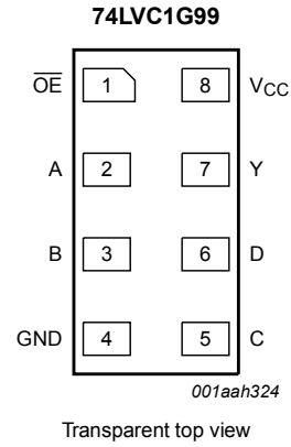
Fig. 3. Pin configuration SOT833-1, SOT1089, SOT1116 and SOT1203 (XSON8)
