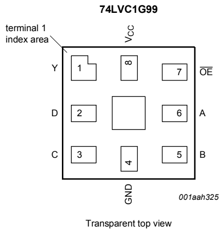
Fig. 3. Pin configuration SOT833-1, SOT1089, SOT1116 and SOT1203 (XSON8)
