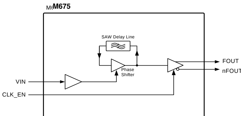
Figure 2: Block Diagram
