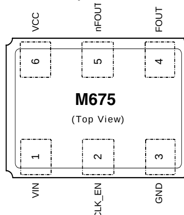
Figure 1: Pin Assignment
