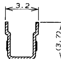
断面 "C"- "C" SECT
