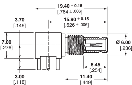
Part Number 1460060-1
