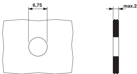
Drilling diagram F-SMA panel feed-through
