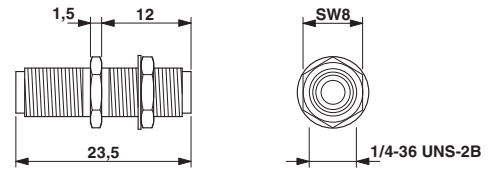
Dimensional drawing F-SMA coupling
