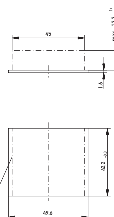
Querplatine / Crosswise circuit board
