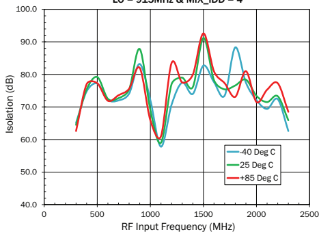
Mixer to Mixer Isolation in Full Duplex Mode LO = 915MHz & MIX_IDD = 4
