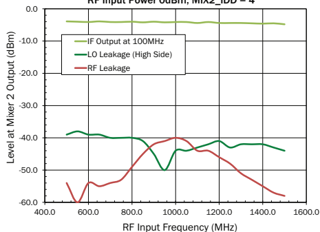
LO & RF Leakage at Mixer 2 Output RF Input Power 0dBm, MIX2_IDD = 4
