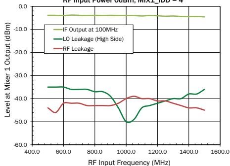
LO & RF Leakage at Mixer 1 Output RF Input Power 0dBm, MIX1_IDD = 4
