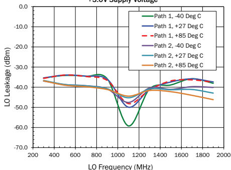
Typical LO Leakage at Mixer Output +3.0V Supply Voltage
