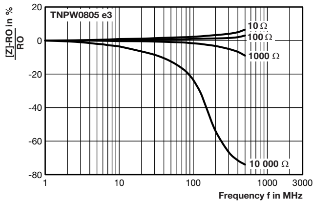
HF Performance (1)
