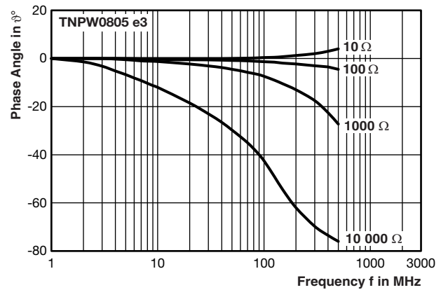
HF Performance (1)
