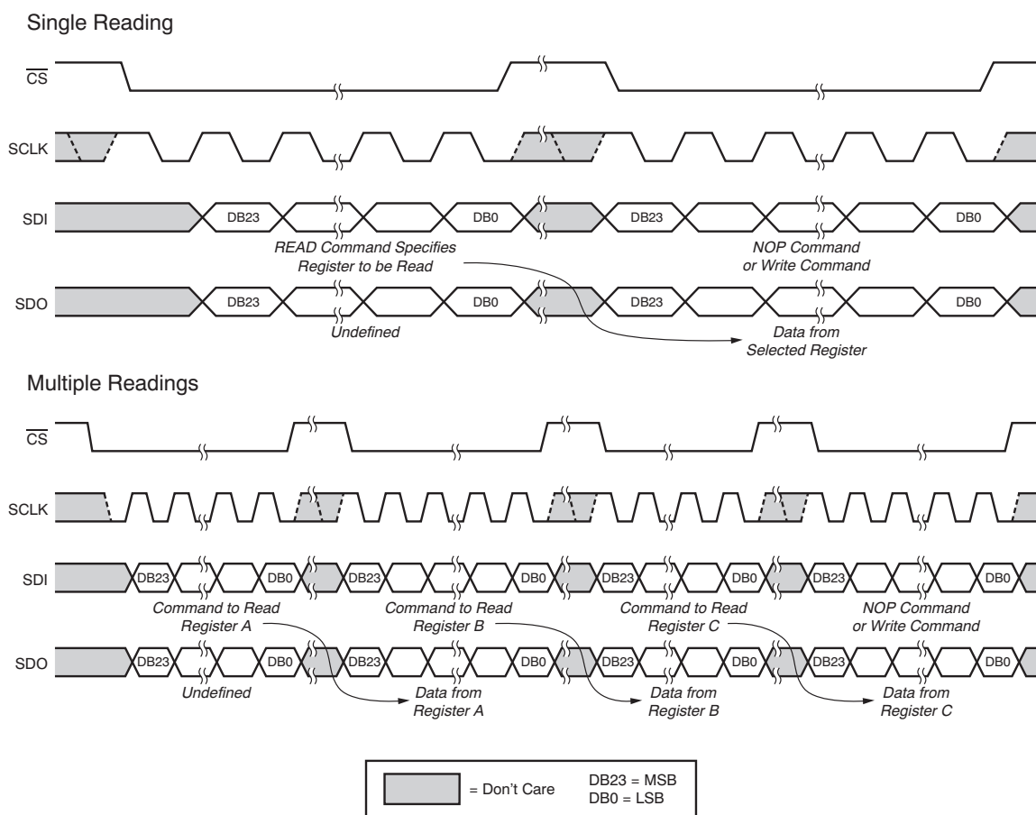
Figure 43. Read-Back Operation
