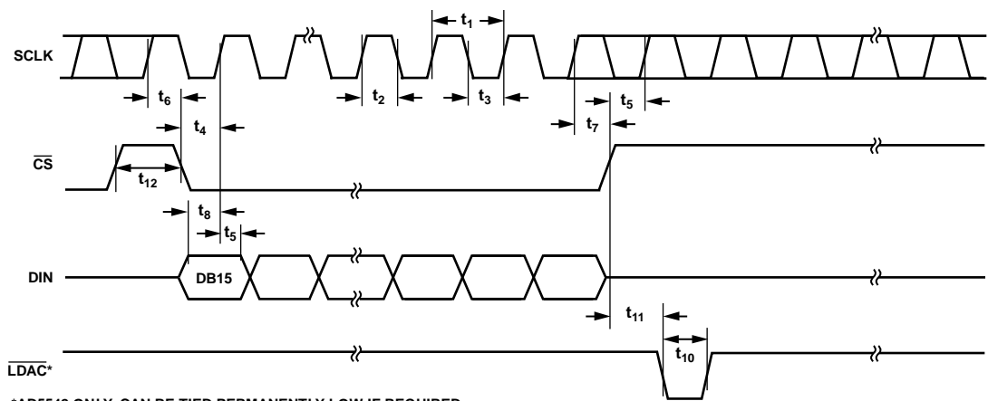
Figure 3. Timing Diagram
