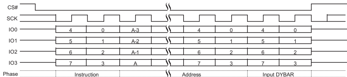
Figure 106. DYBWR QPI Mode Command Sequence [73, 74]
