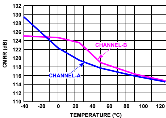
FIGURE 18. ISL28218 CMRR vs TEMPERATURE, V_S = \pm 5V
