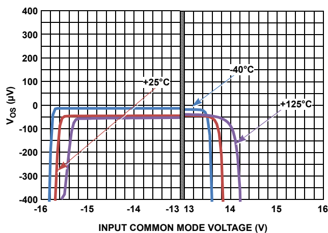
FIGURE 2. INPUT OFFSET VOLTAGE vs INPUT COMMON MODE VOLTAGE, V_S = \pm 15\text{V}
