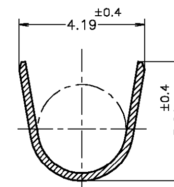
SECT "A"—"A"
