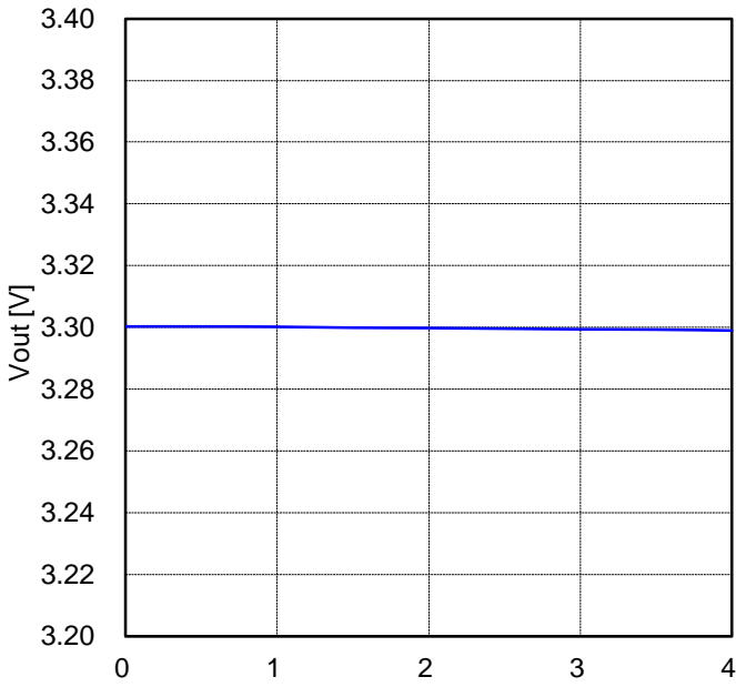
Figure 8. Load Regulation (VIN=12V, Vout=3.3V, L=4.7μH, Cout=44μF)
