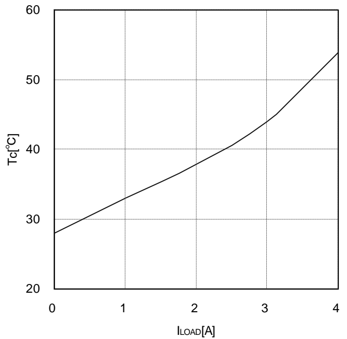
Figure 5. T C VS I LOAD (VIN=12V, Vout=3.3V, L=4.7μH, Cout=44μF)
