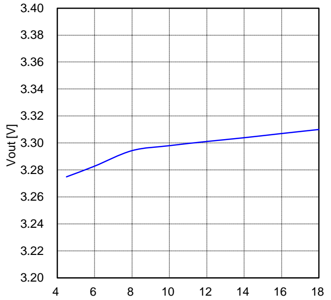
Figure 9. Line Regulation (Vout=3.3V, L=4.7μH, Cout=44μF, Iout=0A)
