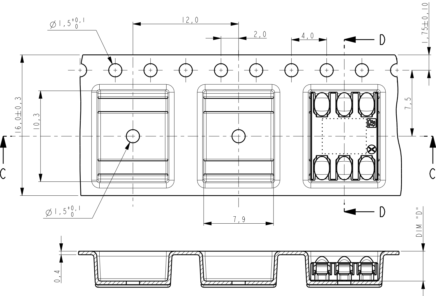
SECTION C-C
