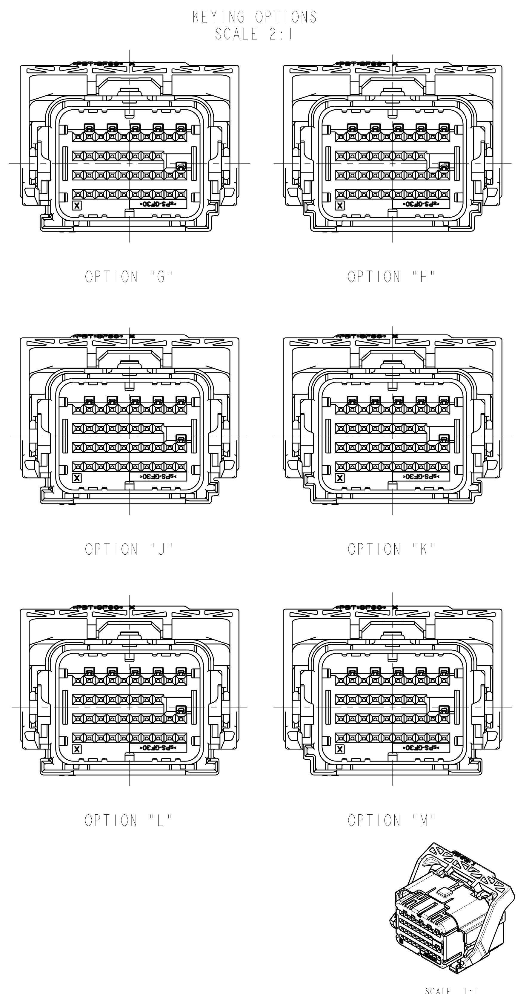
KEYING OPTION "G" SHOWN SEE SHEET 2 FOR BILL OF MATERIALS AND SHEET 3 FOR PIN-OUT CHARTS
