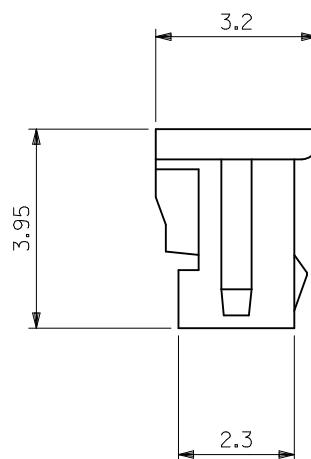
SECT. G-G
