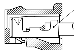
SECT. G-G
