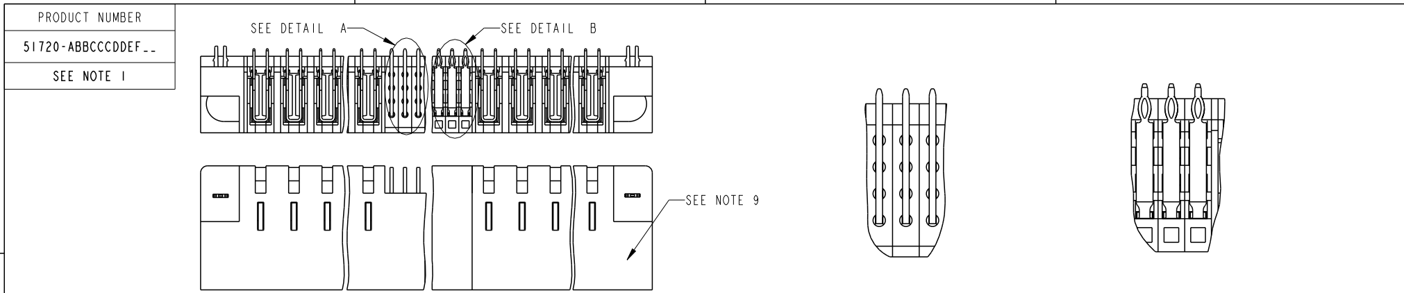
DETAIL A SCALE 2:1 FOR SOLDER TO BOARD ONLY
