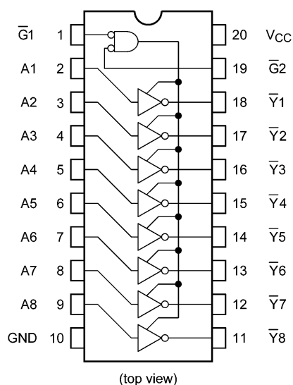
74VHCT540AFT
