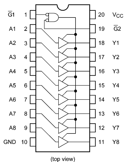
74VHCT541AFT
