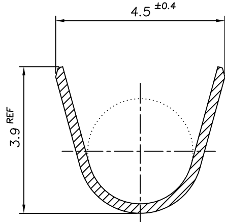
SECTION "D-D" Scale 10/1
