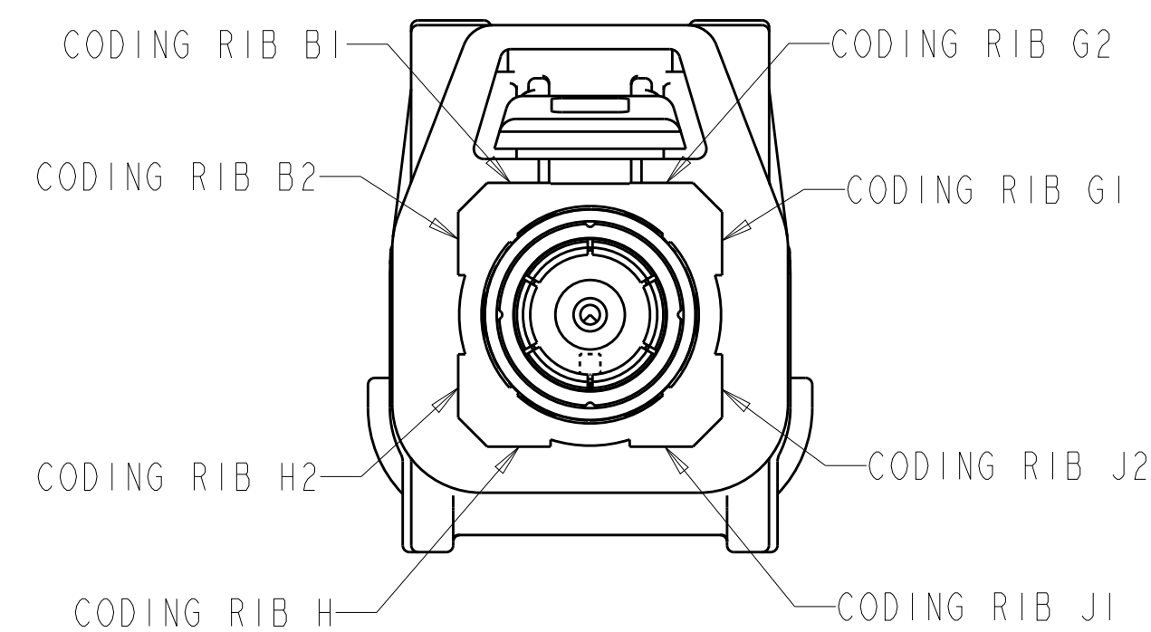
DETAIL Z
