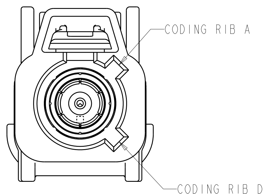
DETAIL D
