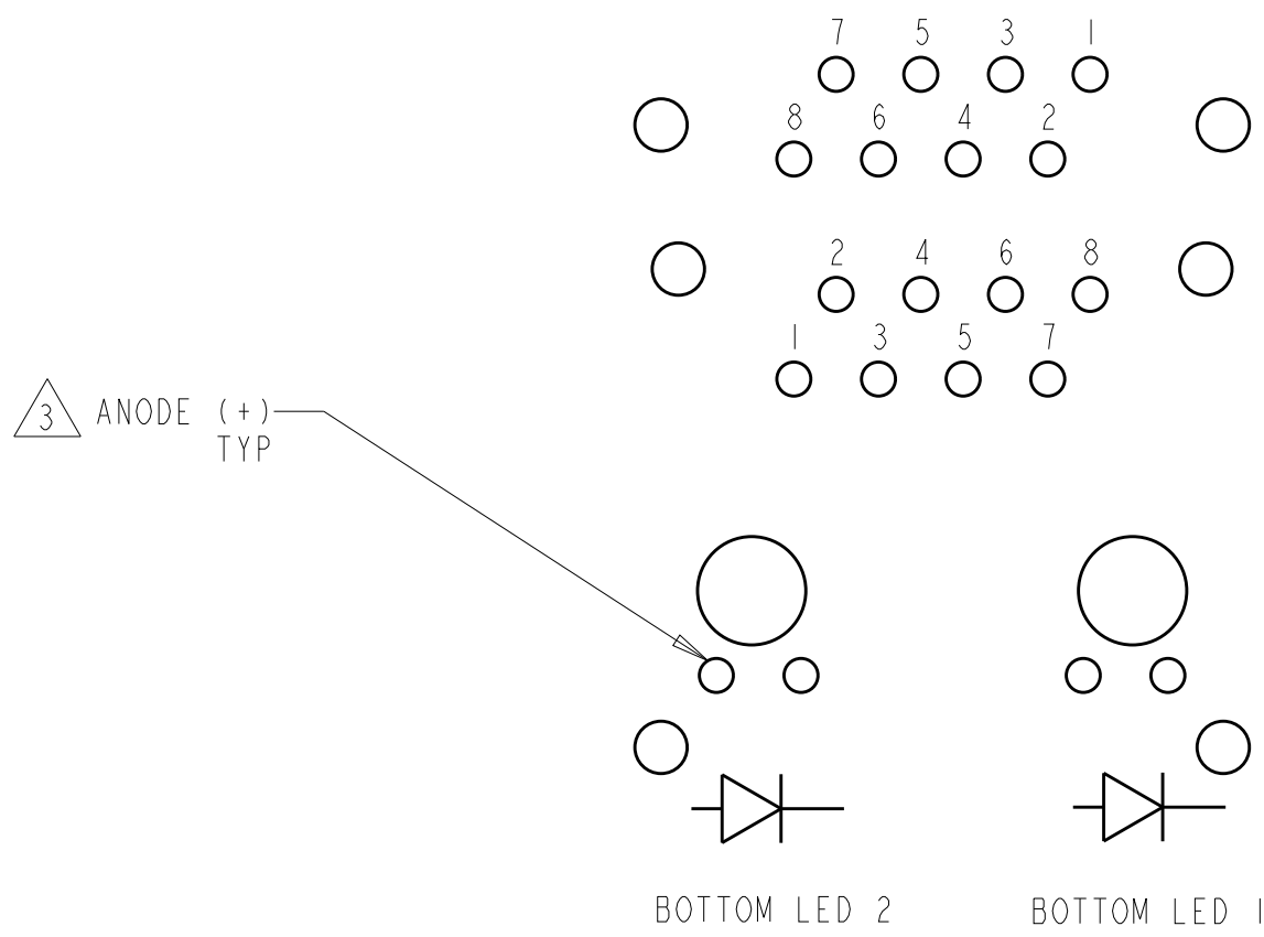
SCHEMATIC FOR 6368011-7, 1-6368011-2, 1-6368011-3
