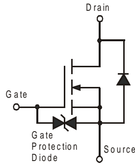
Equivalent Circuit
