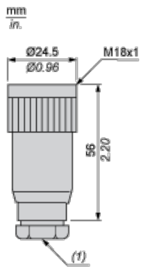
(1) Pg 9 cable gland
