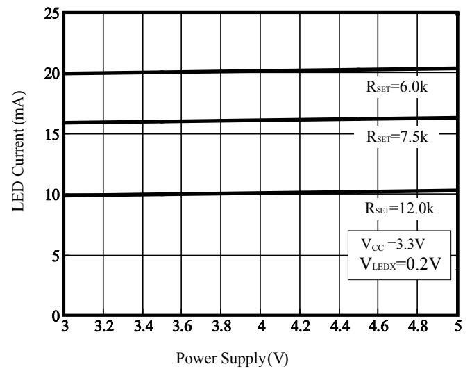
Figure 4 Power Supply vs. LED Current
