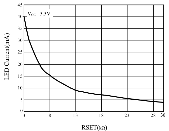
Figure 6 RSET vs. LED Current
