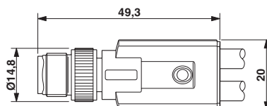
Dimensional drawing
