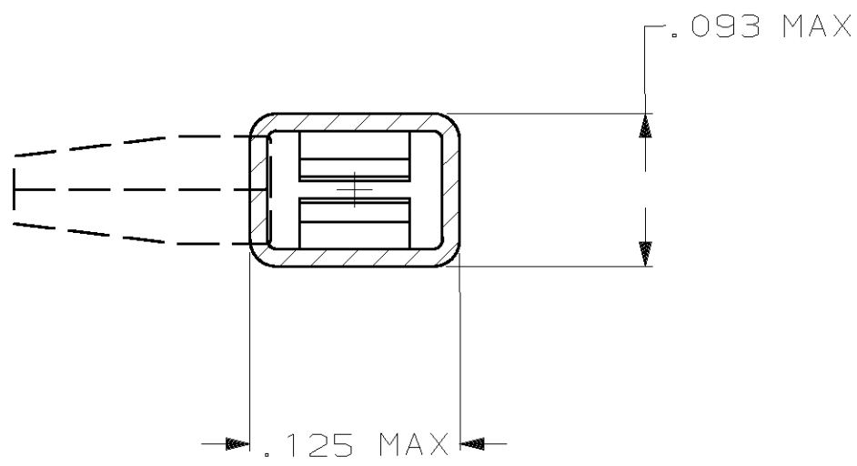
SECTION Y-Y
