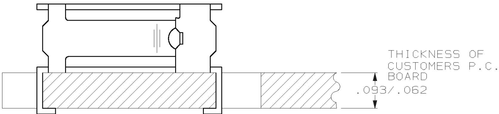
TYPICAL APPLICATION
