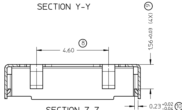
SECTION Z-Z
