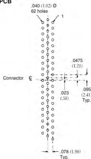
62 High-Density Pin/PCB
