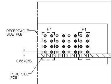
SECTION Z-Z
