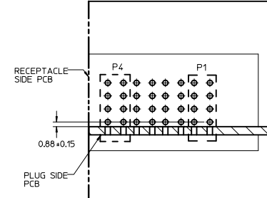
SECTION Z-Z
