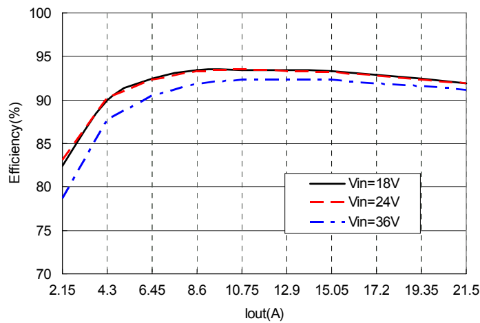
Figure 1 Efficiency vs. output current, T_a=25^{\circ}\text{C} , V_o=28\text{V}
