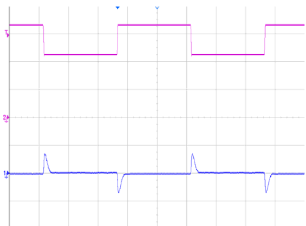
Figure 7 Dynamic response for 25% load step (50% ~ 75% ~ 50%) and 0.1A/μs slew rate, see Figure 13 for test configuration. CH1-output voltage (500mV/div); CH2-output current (5A/div)
