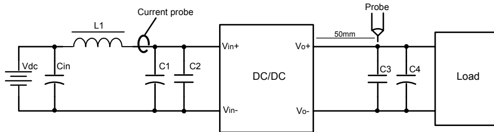
Figure 18 Input ripple & inrush current, ripple & noise test configuration
