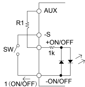
Figure 15 Connection of remote ON/OFF control (B)
