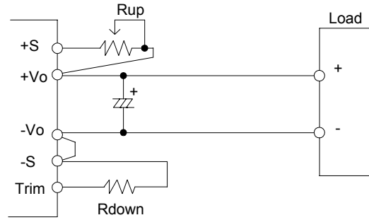
Figure 16 Trim circuit
