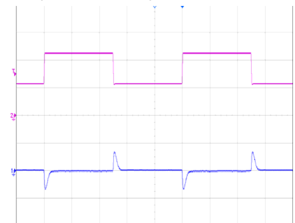
Figure 6 Dynamic response for 25% load step (25% ~ 50% ~ 75%) and 0.1A/μs slew rate, see Figure 13 for test configuration, CH1-output voltage (500mV/div); CH2-output current (5A/div)
