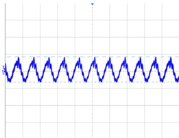
Figure 4 Output ripple & noise (5μs/div, 100mV/div), see Figure 18 for test configuration
