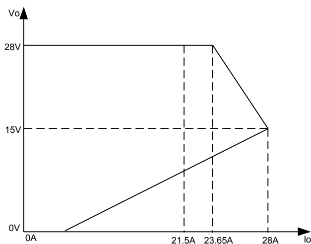
Figure 12 Over-current protection characteristics
