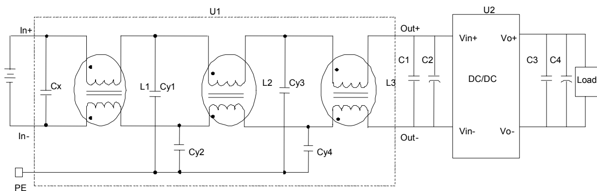
Figure 19 EMC test configuration
