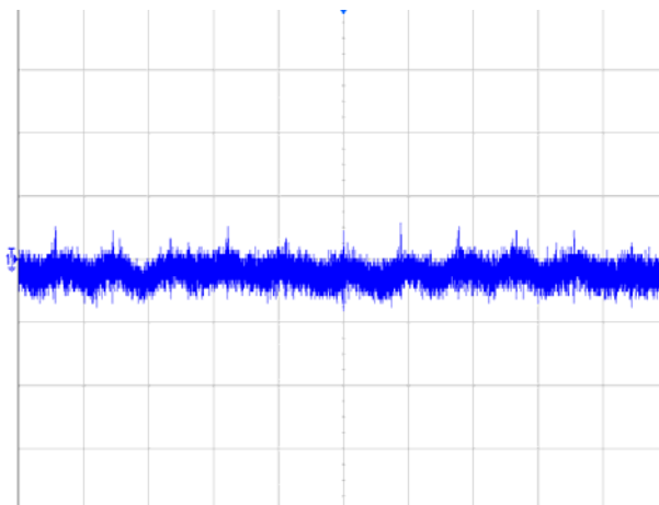
Figure 5 Input reflected ripple current (5μs/div, 20mA/div), see Figure 18 for test configuration
