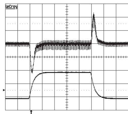
Output voltage response to load current step-change (3.75-11.25-3.75A) at T_{Pcb}=+25\text{ }^{\circ}C , V_{in}=53\text{ V} . Top trace: output voltage (50mV/div.). Bottom trace: load current (5 A/div.) Time scale: 0.1 ms/div.
