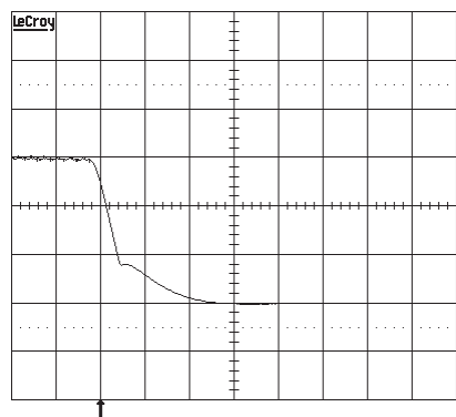
Turn-off at I_o=10A resistive load at T_{Pcb}=+25\text{ }^{\circ}C , V_{in}=53\text{ V} . Turn-off enabled by disconnecting V_{in} . Output voltage (0.5 V/div.). Time scale: 20 \mu s /div.
