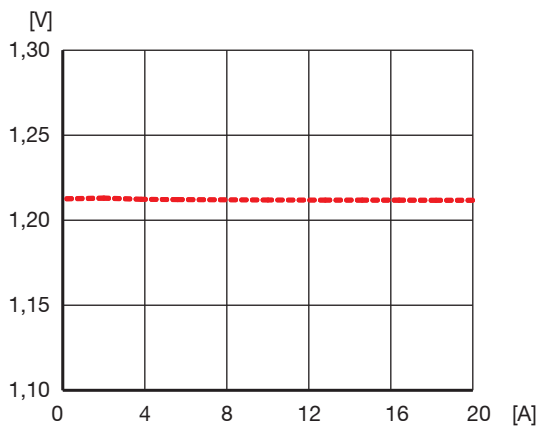
Output voltage vs. load current at T_{Pcb}=+25\text{ °C} , V_{in}=53\text{ V} .
