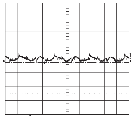
Output voltage ripple (50mV/div.) at T_{Pcb}=+25\text{ }^{\circ}C , V_{in}=53\text{ V} , I_o=10A resistive load with C=10\text{ }μF tantalum and 0.1\text{ }μF ceramic capacitors. Band width=20MHz. Time scale: 2 μs / div.
