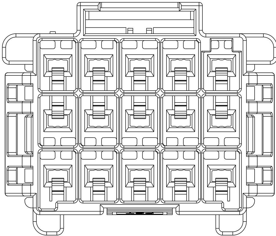
3*5 POSITIONS
