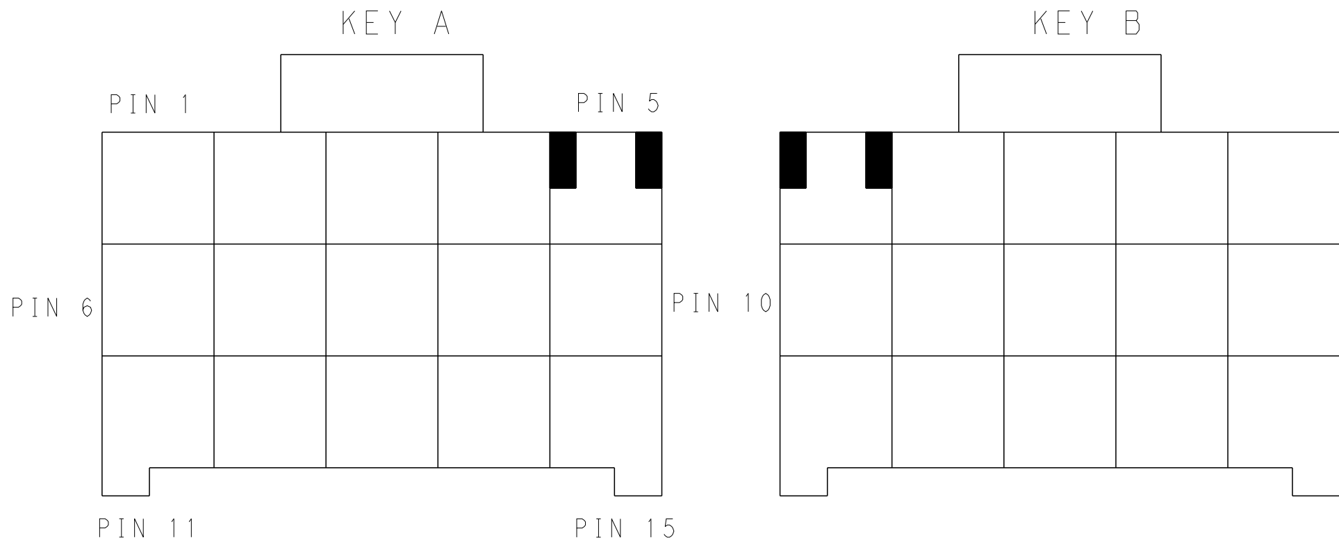
3*5 POSITIONS
