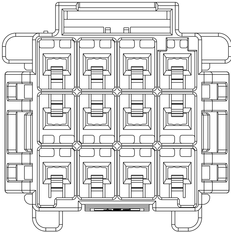
3*4 POSITIONS
