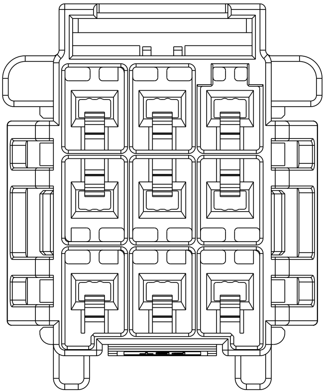
3*3 POSITIONS
