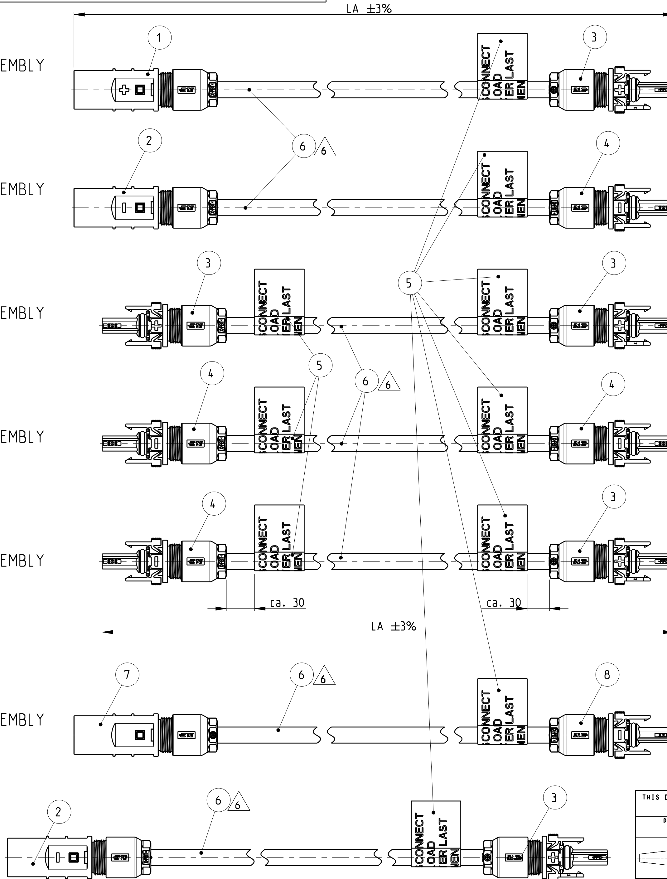
CABLE ASSEMBLY VERSION 7
