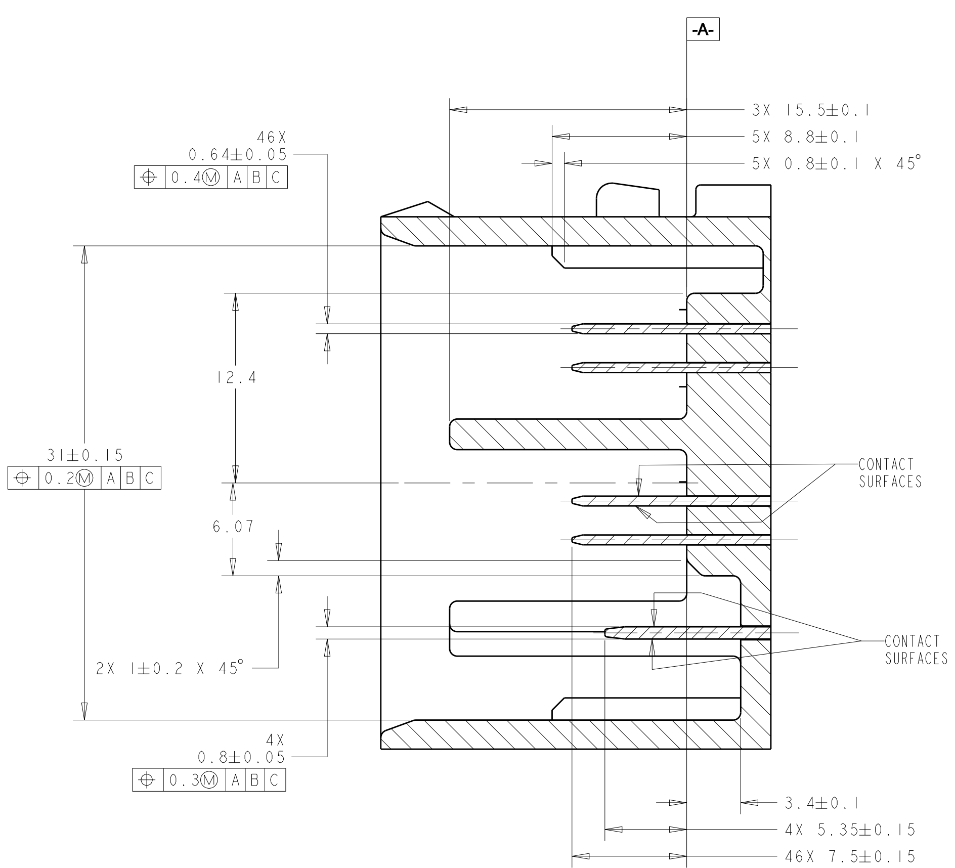
SECTION B-B
