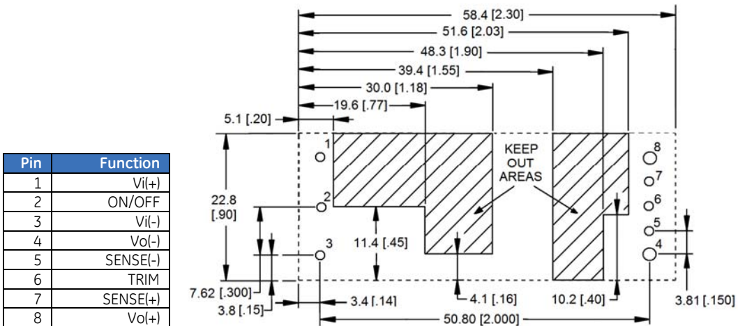
SMT Recommended Pad Layout (Component Side View)
