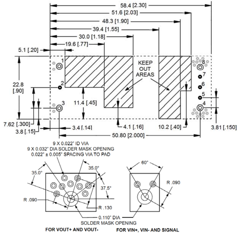
SMT Recommended Pad Layout (Component Side View)
