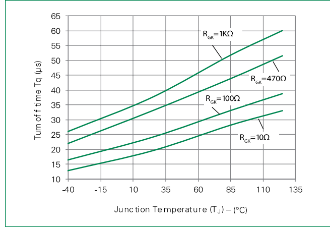
Figure 15-2: Typical turn off time with R_{GK} vs. Junction Temperature for EC103M1
