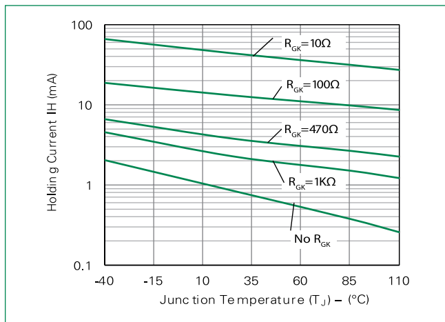
Figure 13-1: Typical DC Holding Current with R_{GK} vs. Junction Temperature for EC103M
