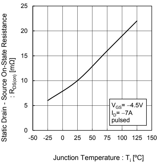
Fig.14 Static Drain - Source On - State Resistance vs. Junction Temperature
