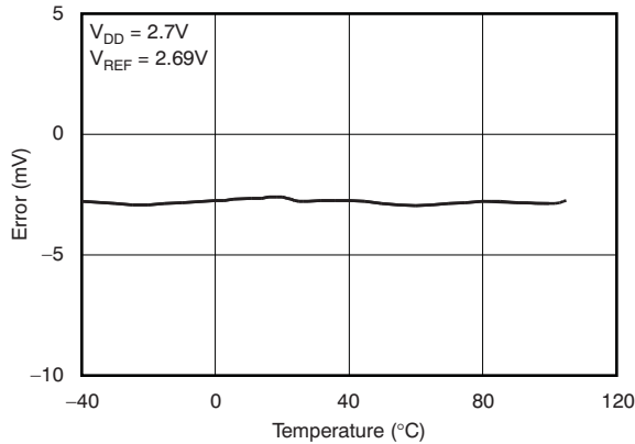
Figure 31. Full-Scale Error vs Temperature
