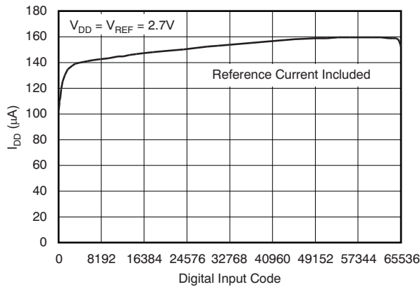
Figure 33. Supply Current vs Digital Input Code
