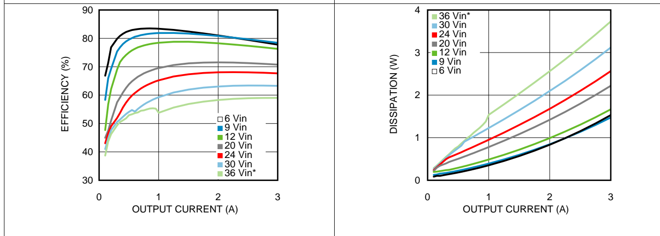
Figure 9. Efficiency 1.8-V Output at 25°C Ambient
