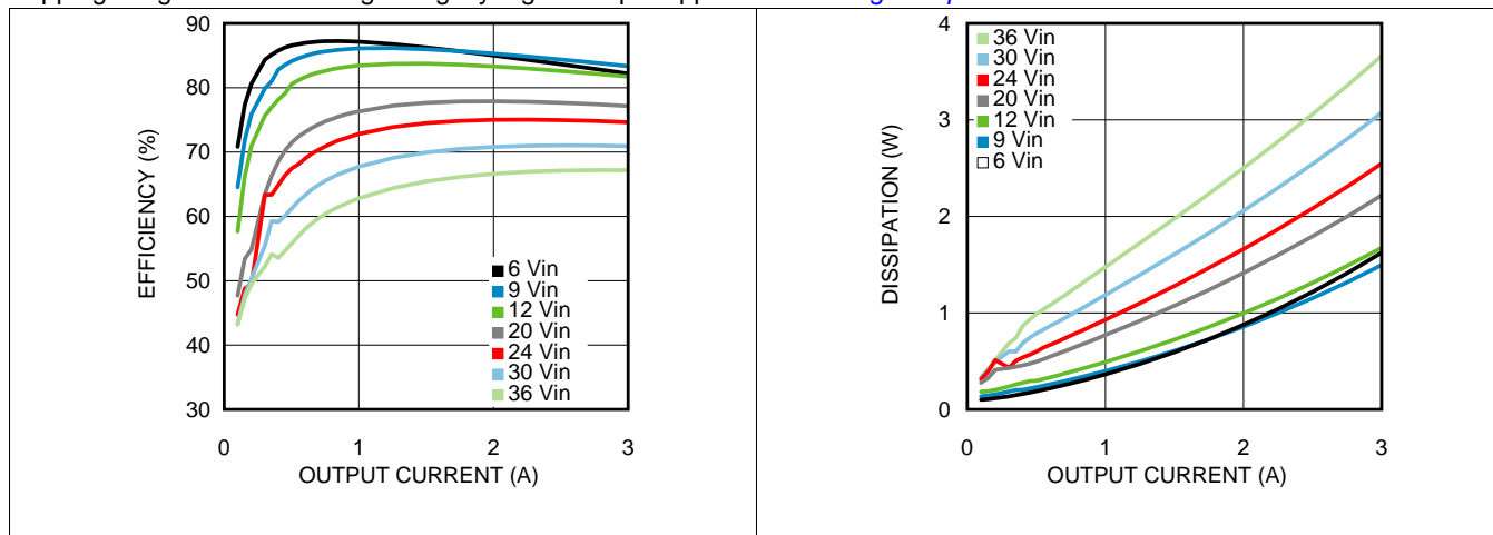
Figure 7. Efficiency 2.5-V Output at 25°C Ambient
