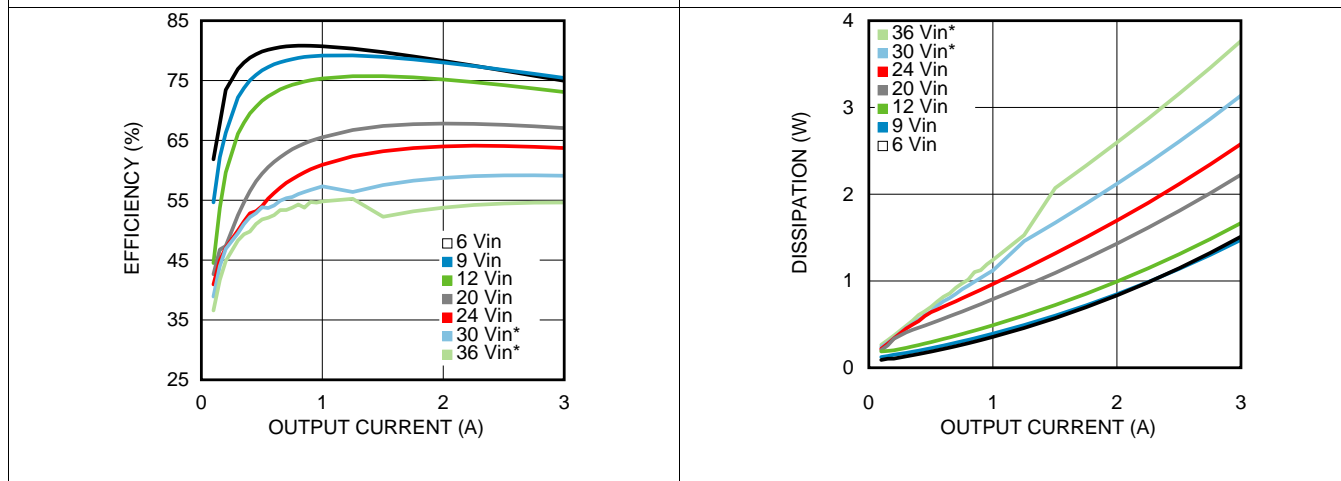
Figure 11. Efficiency 1.5-V Output at 25°C Ambient
