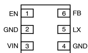
Figure 6. Pin Connections – UDFN6
