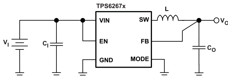
Figure 24. Measurement Setup
