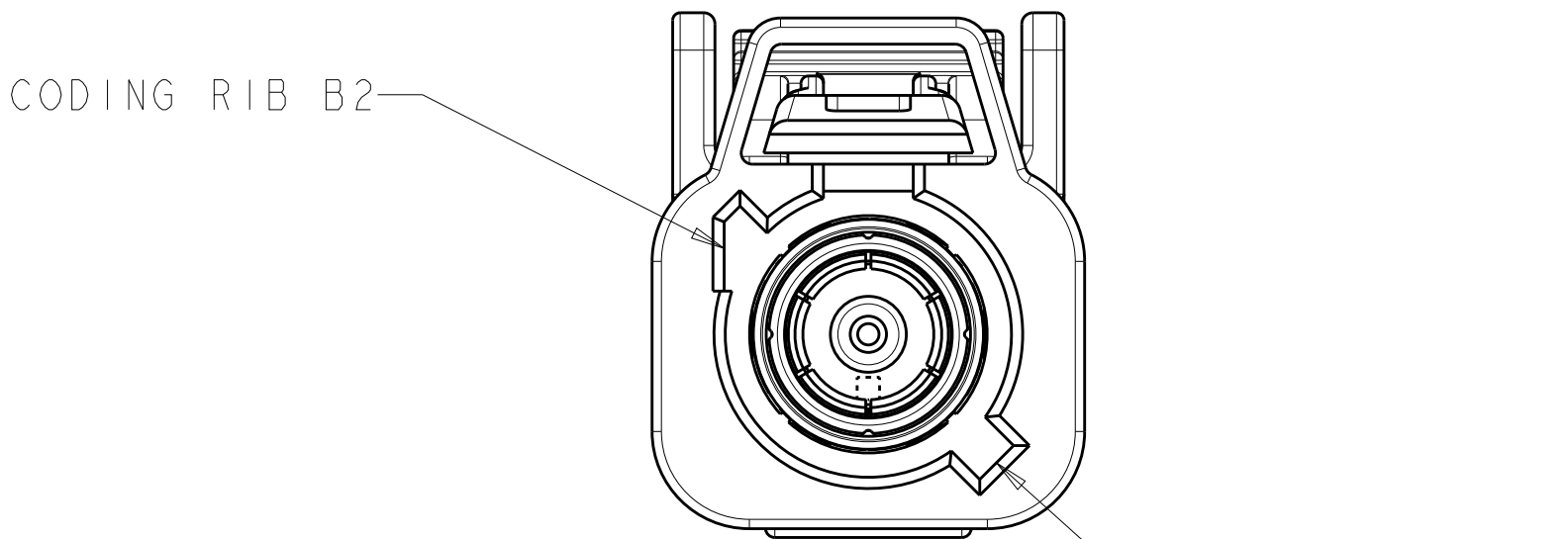
DETAIL I
