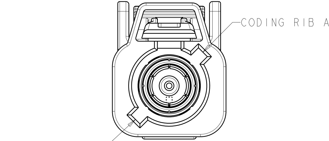
DETAIL C
