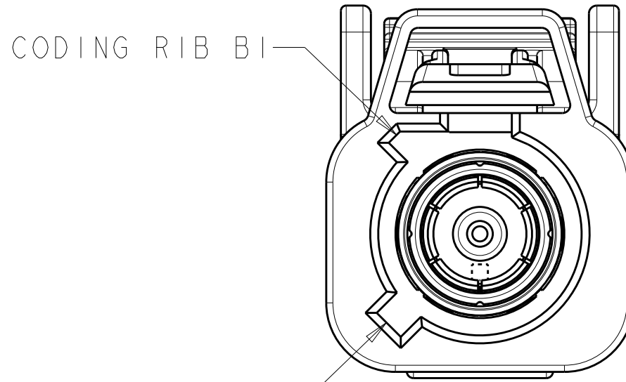
DETAIL F
